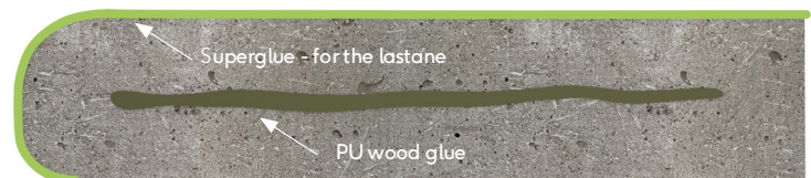
Location of glue on mitres
