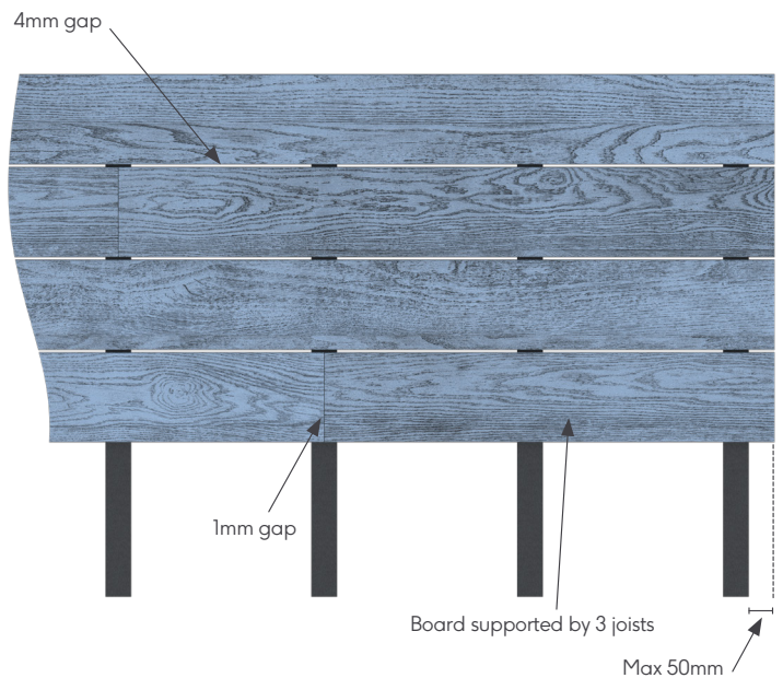
General gapping on boards
