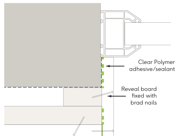
Fig. 17 - Window/ door jamb with Reveal board - brad nails
