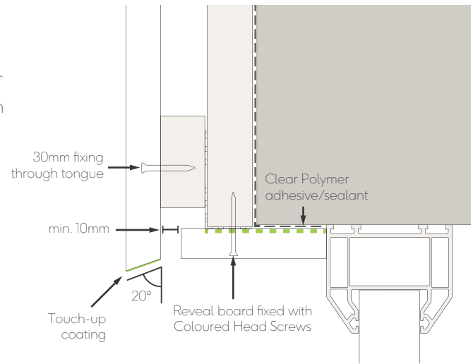
Fig. 15 - Window/door head with angled cut
